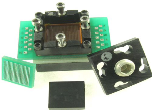
Figure 1: GHz BGA Socket
